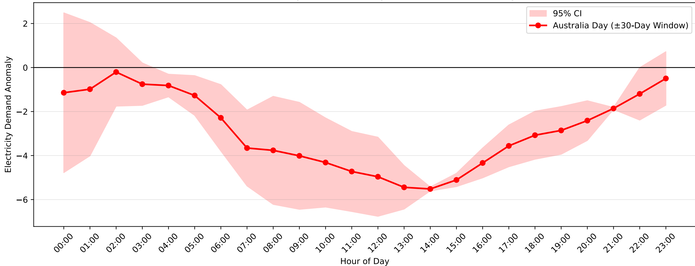
Cardiff Demand Anomaly: Australia Day (2008–2009, \pm 30 -Day Window)
